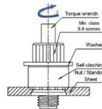
Torque-out
