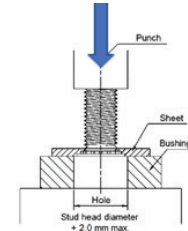
Pushout
